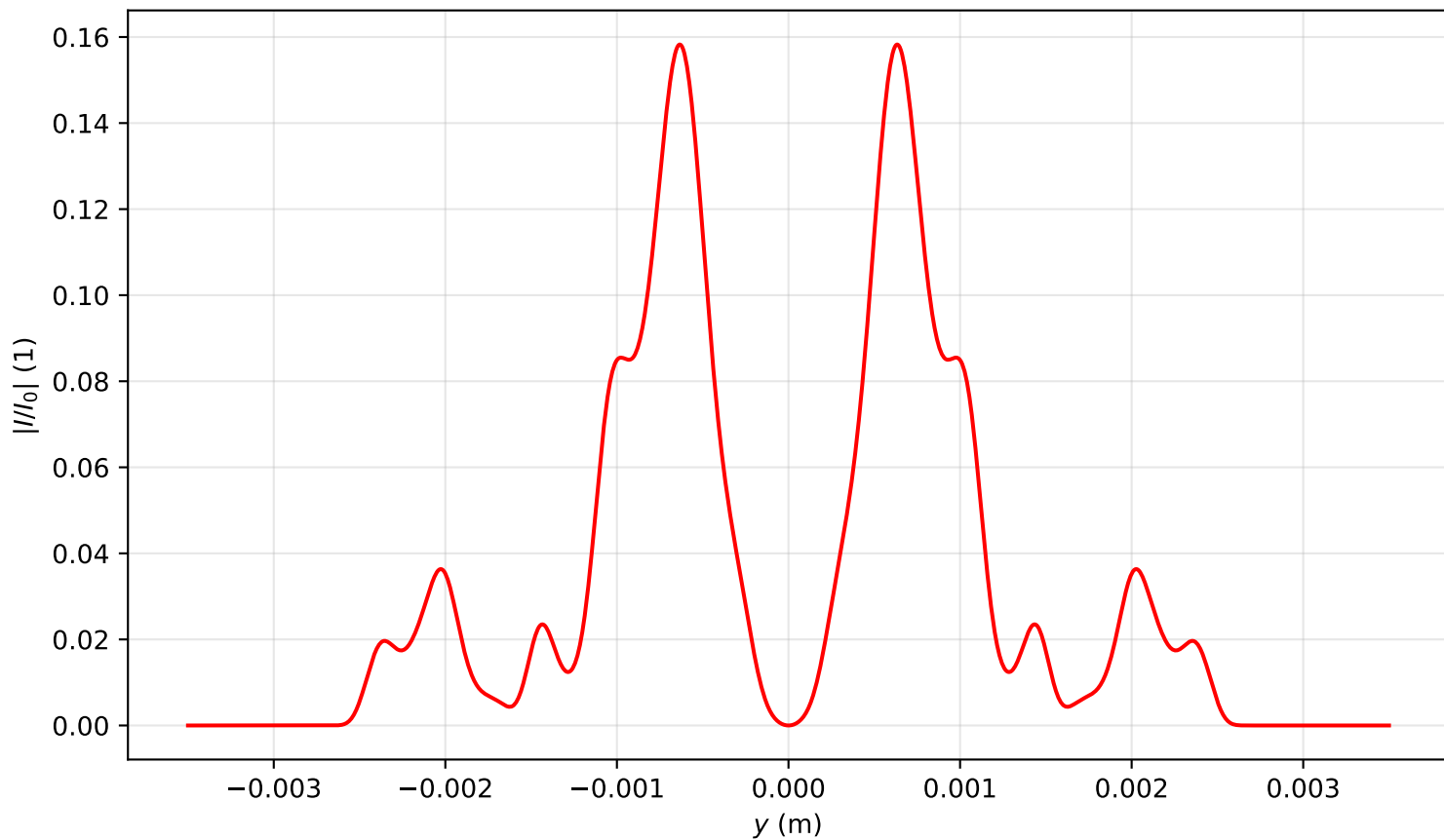
Intensity profile I(x=0, y, z=2.866)/I_0 , \text{Pin}=9.0\text{Pcr} , artificial time
